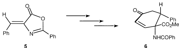
Scheme 1. Synthesis of \alpha,\beta -unsaturated compound 6 from 5(4H)-oxazolone 5
